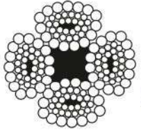
U4x39 + SES Dönmez - Swaged Galvaniz
