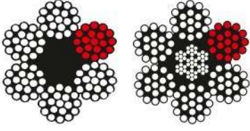
6x19 Standart (TS 1918/10)
