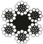
6x19 & 6x26 Warrington Seale L.Öz (TS 1918/11)
