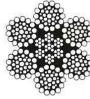
6x36 WS Ç.Öz (TS 1918/14)
