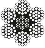
6x25 + (7x7) WS FİLLER
